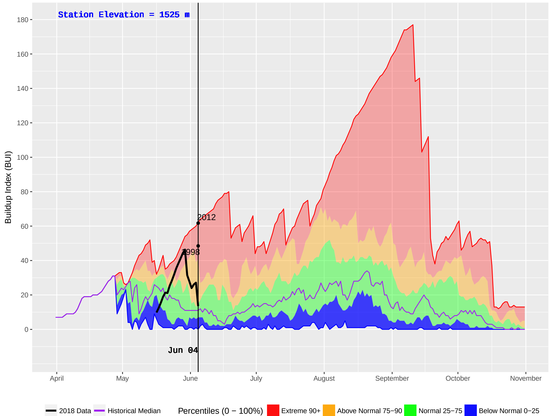
HARBOUR LAKE (250) : Historical (1989–2016) and Current (2018) Noon Buildup Index (BUI)
